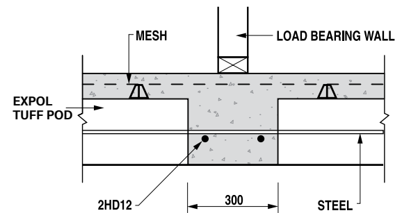
Fig 7.5 300mm Rib
